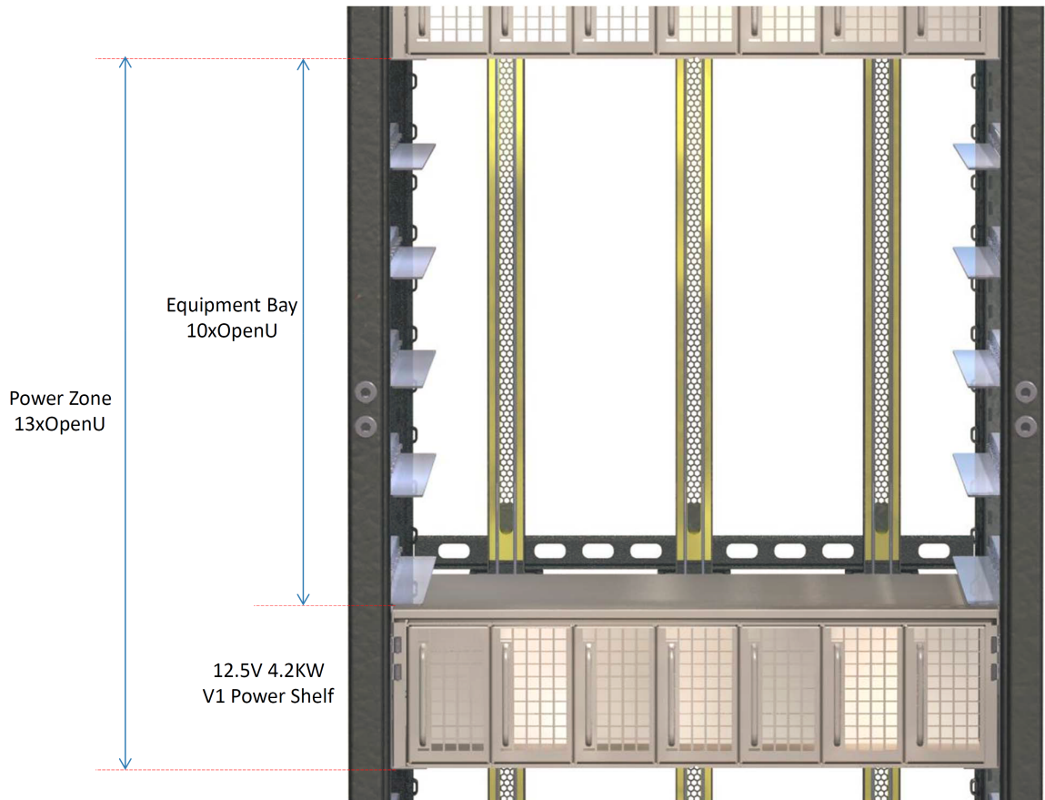
Figure 8 Power Zone: 3xOpenU Power Shelf + 10xOpenU Equipment Bay
