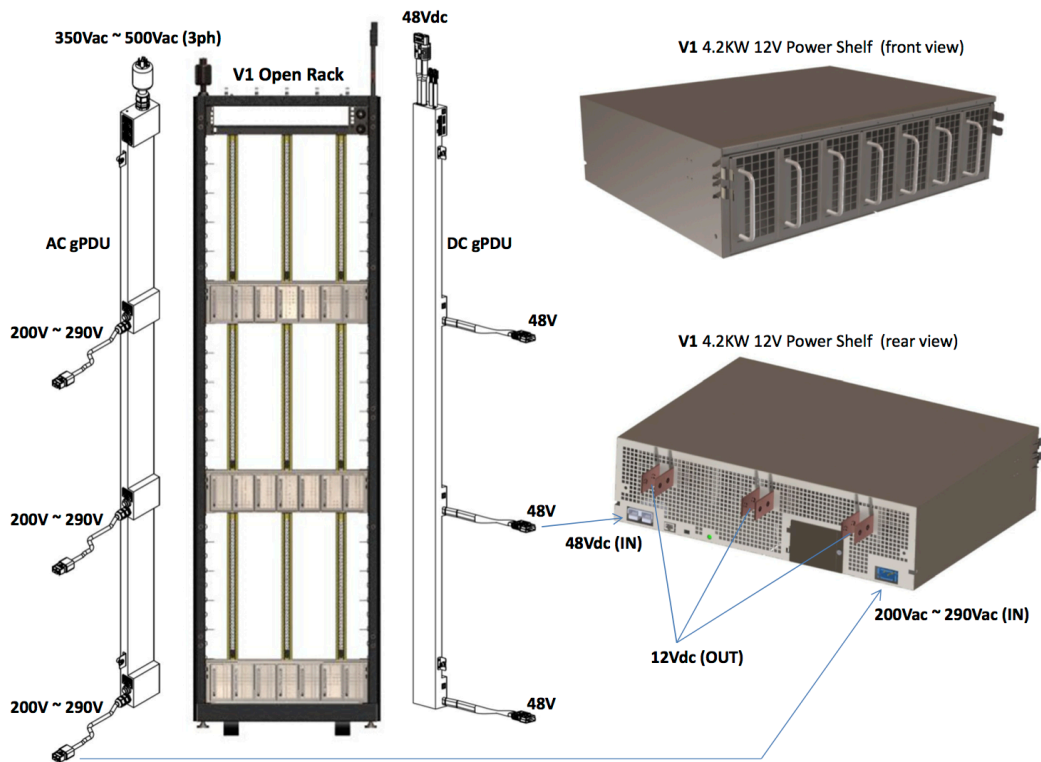
Figure 6 V1 Power Shelf and PDU Components
