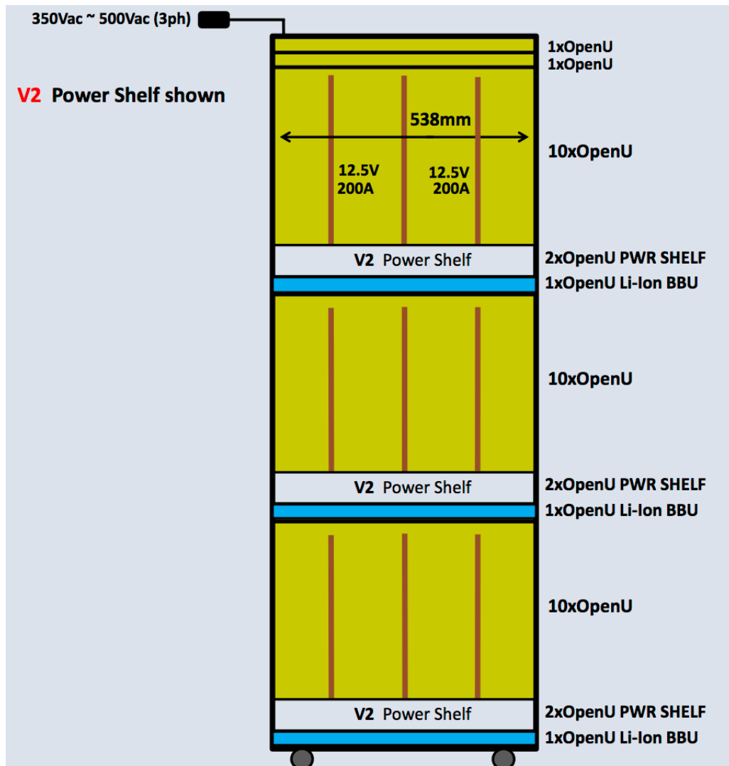
Figure 5 Open Rack with 2xOpenU Power Shelf and 1xOpenU BBU
