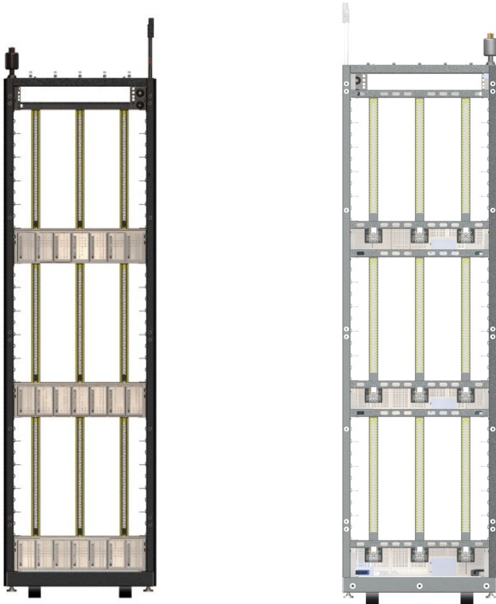
Figure 7 Open Rack with PDUs (Front View, Left; Rear View, Right)
