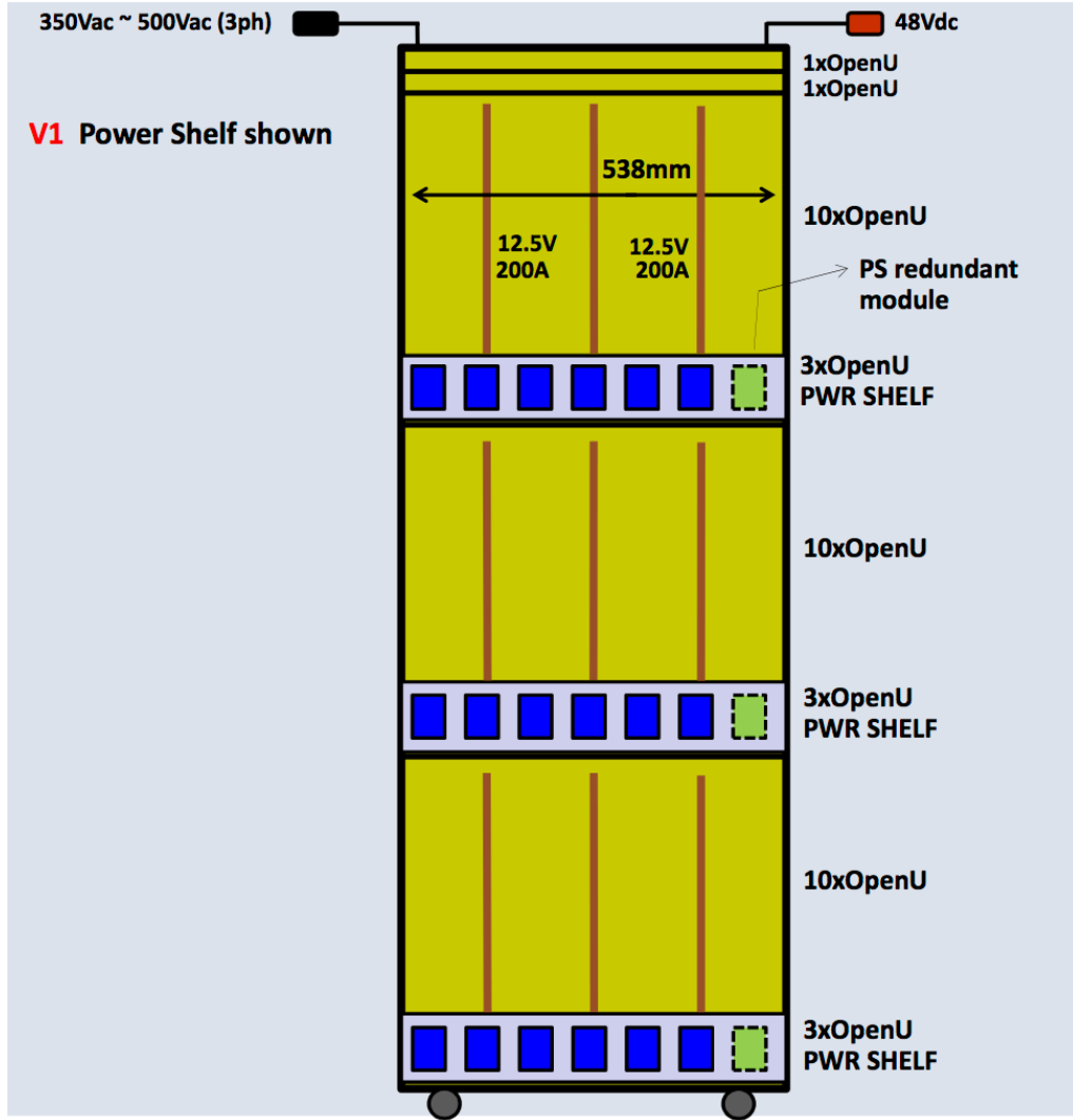
Figure 4 Open Rack with Three 3xOpenU V1 Power Shelves (OCP Battery Cabinet not Shown)
