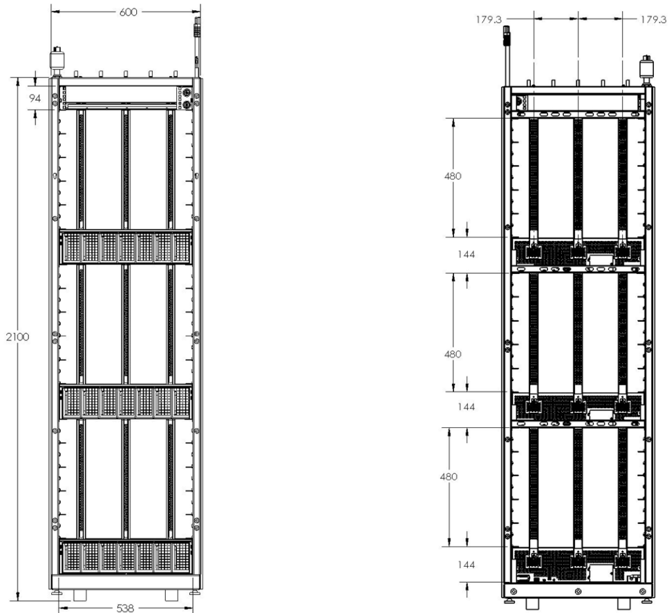
Figure 2 Open Rack Structural Drawing with PDUs (Front View, Left; Rear View, Right)
